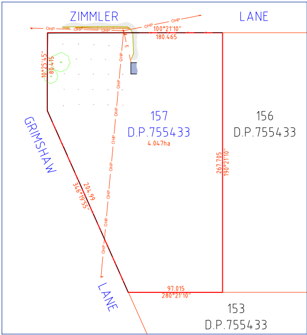
SITE DIAGRAM SCALE 1:2000 (A1) 1:4000 (A3)
