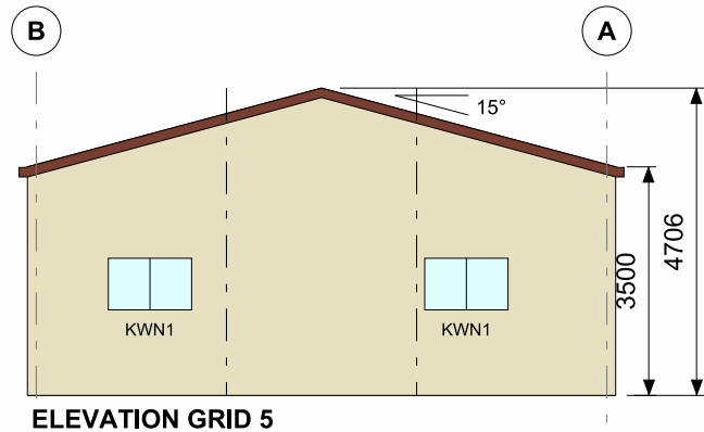
ELEVATION GRID 5
