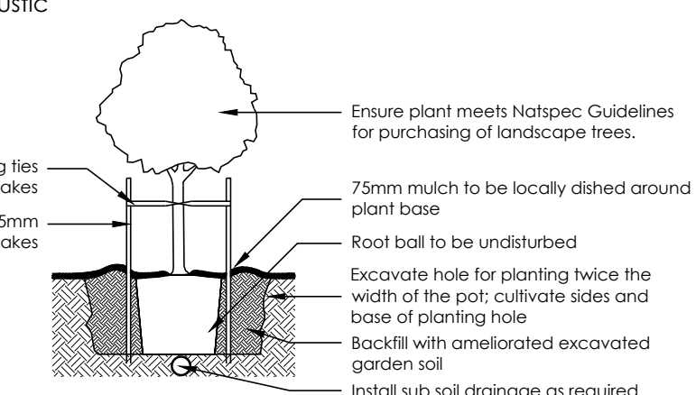
1 Tree Planting Detail NTS 25L - 75L Pot Size
