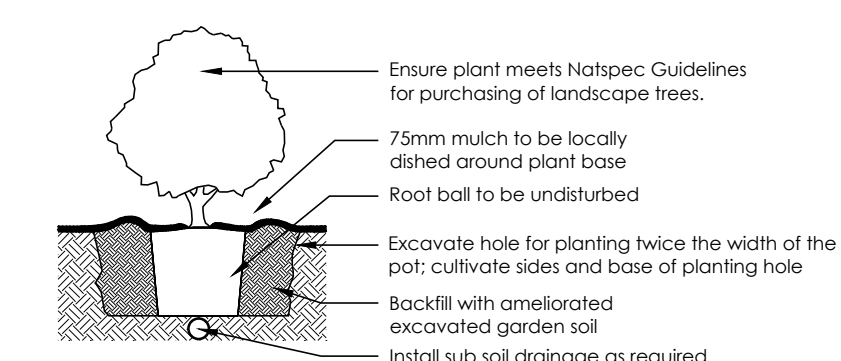
2 NTS Planting Detail Tube, 150mm, 200mm Pot Size
