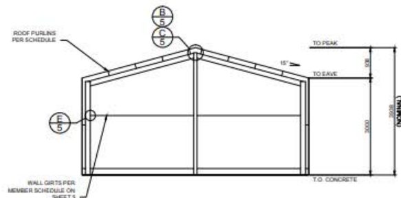
3 2 ENDWALL INTERIOR ELEVATION SCALE: 1 = 100
