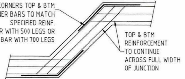
BEAM BAY WINDOW INTERSECTION PLAN
