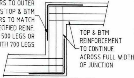
BEAM "L" INTERSECTION PLAN
