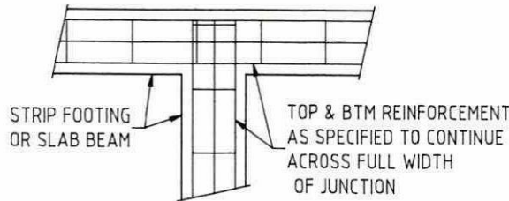
BEAM "T" INTERSECTION PLAN
