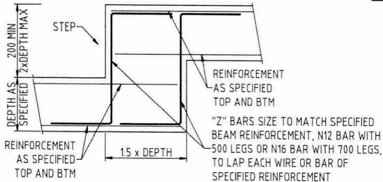
STRIP FOOTING STEPPING DETAILS
