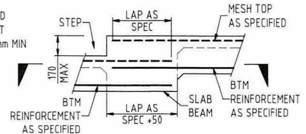
CONTINUOUS SLAB BEAMS WITH DIFFERENT FOUNING LEVELS
