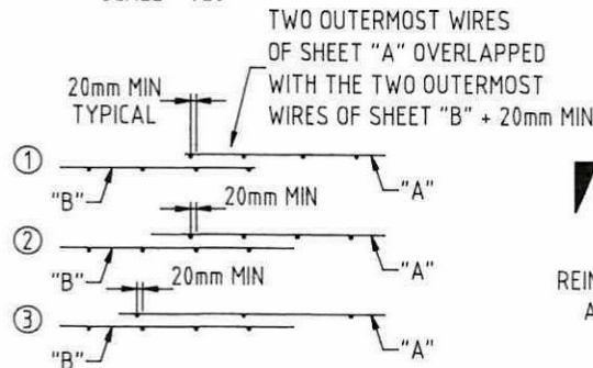
MESH LAPPING DETAILS
