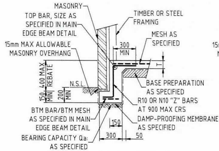
400mm MAX REBATE - OPTION 1
