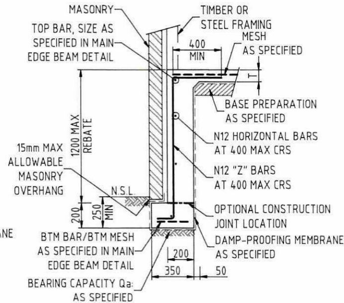
1200mm MAX REBATE
