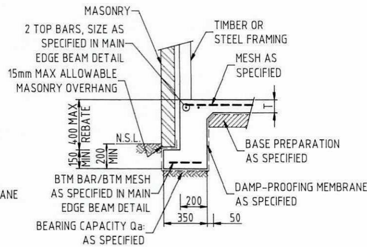
400mm MAX REBATE - OPTION 2
