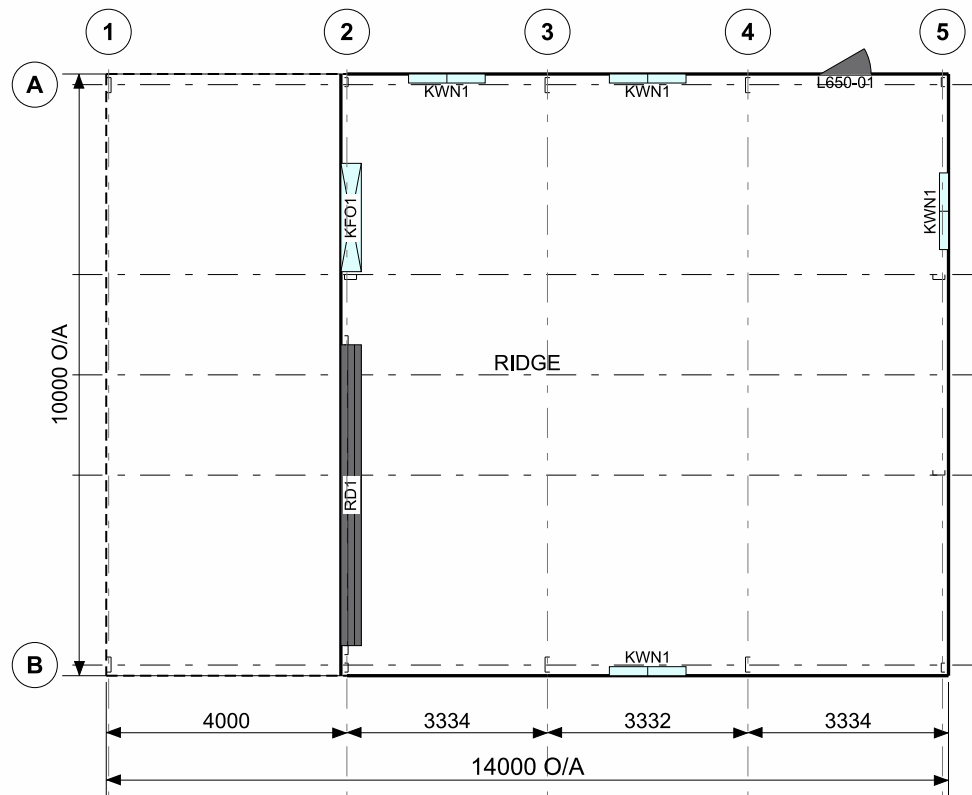
FRAME ROOF PLAN
