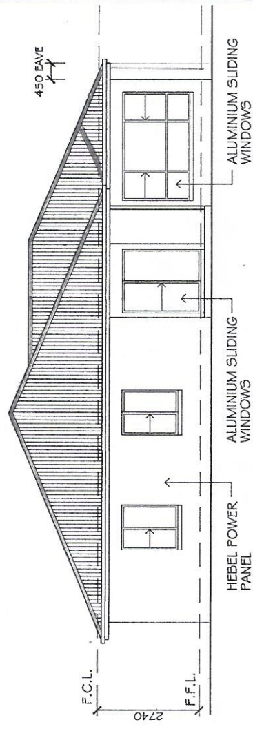
SOUTH ELEVATION
