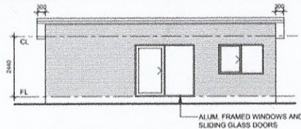
1 FRONT ELEVATION
