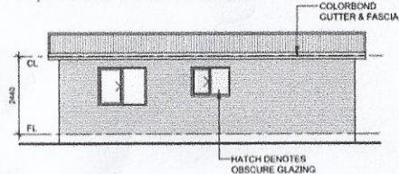
3 REAR ELEVATION
