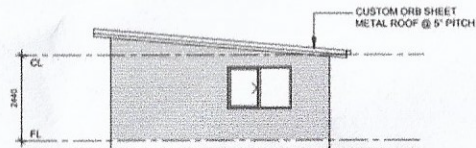
4 SIDE ELEVATION
