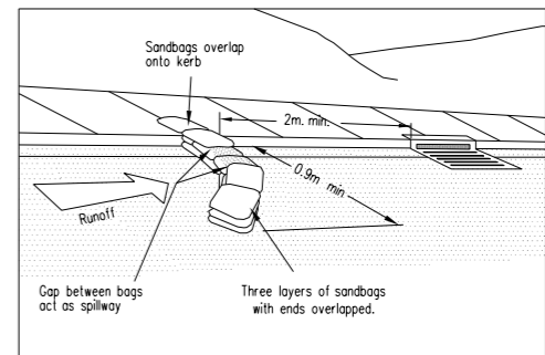
Sandbag Kerb Inlet Sediment Trap
