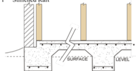
Fig. 1 Stiffened Raft
